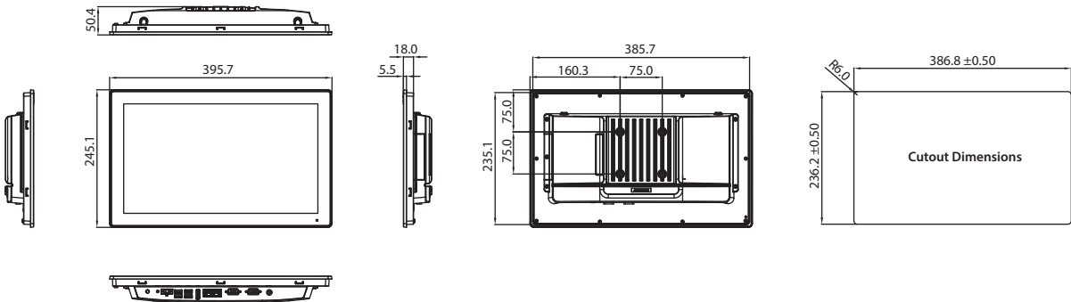
Panel Cutout Dimensions: 386.8 x 236.2 mm (15.23 x 9.30 in)
