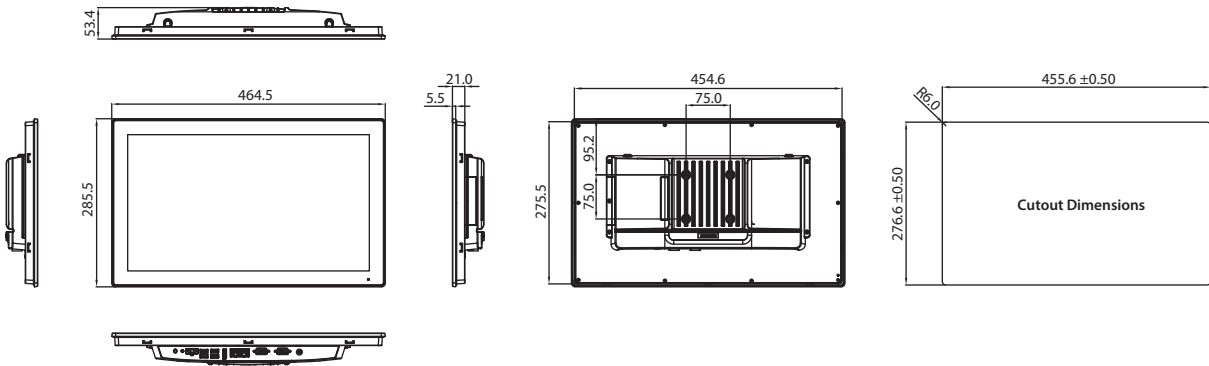
Panel Cutout Dimensions: 455.6 x 276.6 mm (17.94 x 10.89 in)
