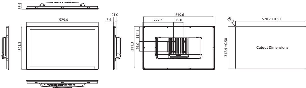
Panel Cutout Dimensions: 520.7 x 312.4 mm (20.5 x 12.3 in)
