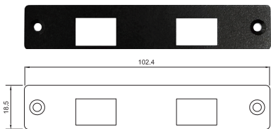
UB1328 Universal Bracket with 2 x RJ45 Cutout Dimension (WxD): 102.4 x 18.5 mm
