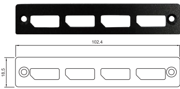
UB1329 Universal Bracket with 4x DP Cutout Dimension (WxD): 102.4 x 18.5 mm
