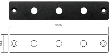
UB0932 Universal Bracket with 3x Antenna Cutout Dimension (WxD) : 96.95 x 18.4 mm
