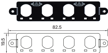
UB0710 Universal Bracket with 4x M12 Cutout Dimension (WxD) : 82.5 x 19.5 mm
