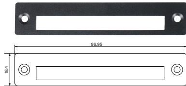
UB1318 Universal Bracket with DIO Cutout Dimension (WxD): 96.95 x 18.4 mm
