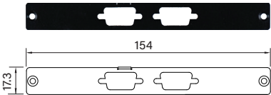
UB0503 Universal Bracket with 2x DB9 Cutout Dimension (WxD) : 154 x 17.3 mm
