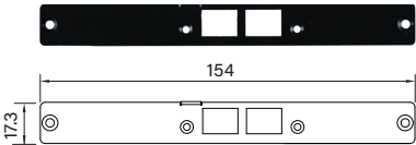
UB0511 Universal Bracket with 2x RJ45 Cutout Dimension (WxD) : 154 x 17.3 mm
