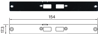
UB0514 Universal Bracket with 2x USB Cutout Dimension (WxD) : 154 x 17.3 mm
