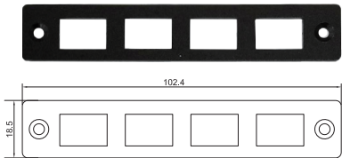
UB1312 Universal Bracket with 4x RJ45 Cutout Dimension (WxD): 102.4 x 18.5 mm
