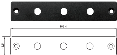
UB1332 Universal Bracket with 3x Antenna Cutout Dimension (WxD): 102.4 x 18.5 mm
