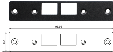
UB1311 Universal Bracket with 2x RJ45 Cutout Dimension (WxD): 96.95 x 18.4 mm
