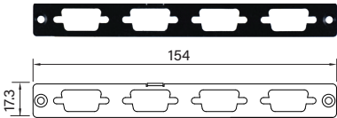
UB0504 Universal Bracket with 4x DB9 Cutout Dimension (WxD) : 154 x 17.3 mm
