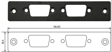
UB1303 Universal Bracket with 2x DB9 Cutout Dimension (WxD): 96.95 x 18.4 mm
