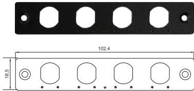
UB1310 Universal Bracket with 4x M12 Cutout Dimension (WxD): 102.4 x 18.5 mm
