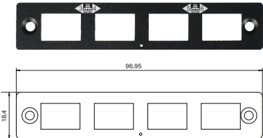
UB0912 Universal Bracket with 4x RJ45 Cutout Dimension (WxD) : 96.95 x 18.4 mm
