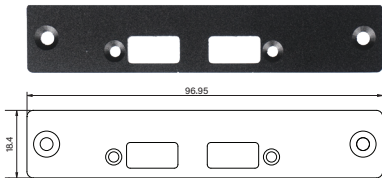
UB1314 Universal Bracket with 2x USB Cutout Dimension (WxD): 96.95 x 18.4 mm
