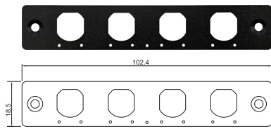
UB1330 Universal Bracket with 4x M12 X-Coded Cutout Dimension (WxD): 102.4 x 18.5 mm
