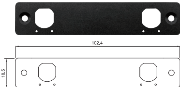
UB1337 Universal Bracket with 2x M12 X-coded Cutout Dimension (WxD): 102.4 x 18.5 mm
