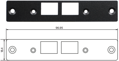
UB0911 Universal Bracket with 4x M12 Cutout Dimension (WxD) : 96.95 x 18.4 mm
