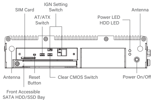
Front I/O
