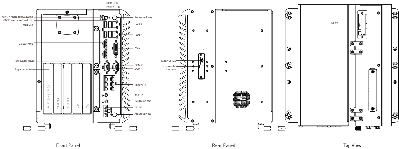
Front Panel
