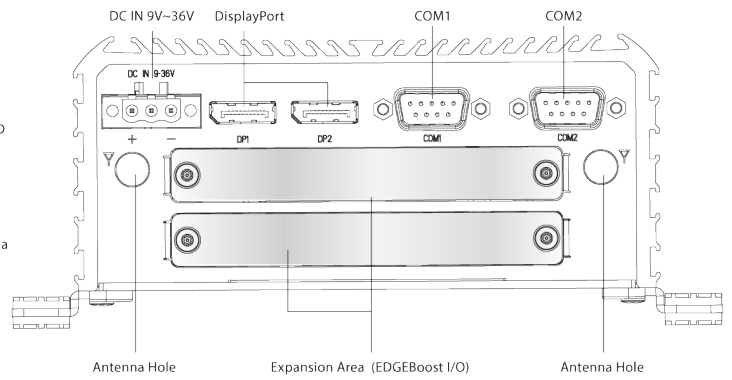
Rear Panel
