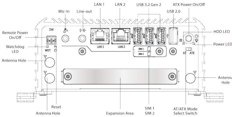
Front Panel
